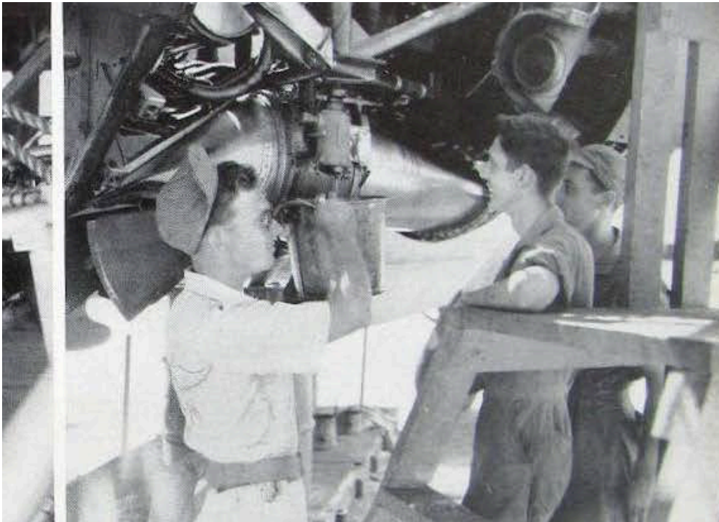
380 th Sub Depot personnel draining the oil in a B-26 engine.(USAAF photo)
